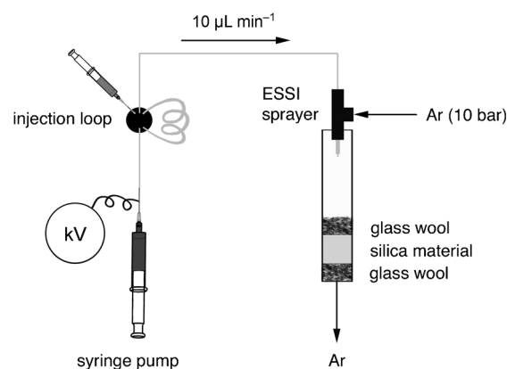
Figure 1. Synthesis using an electrosprayer enclosed in a polypropylene vessel bottom sealed with glass wool and silica. The high voltage was applied through the stainless steel needle of the syringe, while a grounded aluminum foil covered the vessel.
