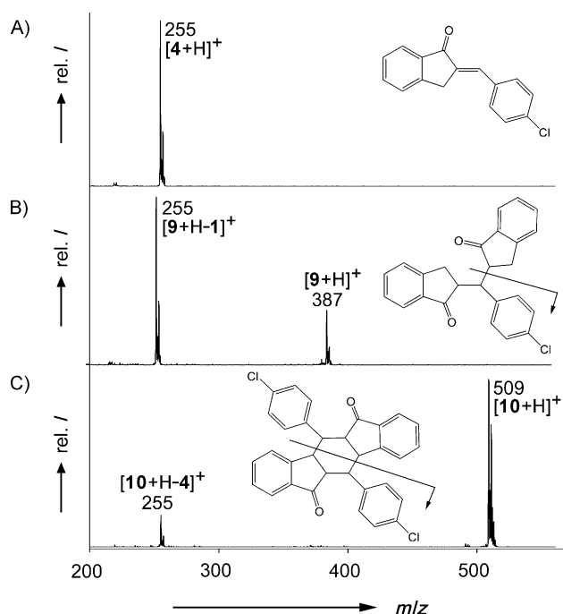
Figure 4. APCI-MS spectra of A) the main product 4 and B) the side product 9 as well as C) the side product 10 obtained from a preparative electrospray. The insets show the corresponding structural formulae and key fragments; rel. I = relative intensity.
