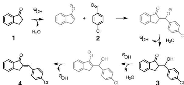
Scheme 1. Mechanism of the base-catalyzed Claisen–Schmidt condensation of 1-indanone ( 1 ) and 4-chlorobenzaldehyde ( 2 ) to 2-(4-chlorobenzylidene)indan-1-one ( 4 ). Negatively charged intermediates are drawn in grey.
