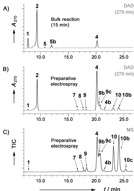
Figure 3. HPLC-APCI-MS product analysis with UV detection (DAD) at 270 nm: A) reaction mixture and B) product of the preparative electrospray. C) Total ion current (TIC) chromatogram for the HPLC analysis depicted in (B). For more details see Figure S2 and Tables S2 to S5 in the Supporting Information.
