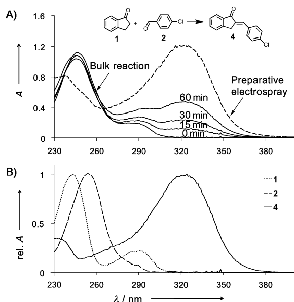
Figure 2. A) Time course of reactions in bulk solution (solid lines analyzed after 0, 15, 30, and 60 min) and in preparative electrospray after 10 min of spraying. Analysis is done by UV/Vis spectroscopy and the spectra are normalized to equal amounts of reagents 1 and 2 ( A = absorbance). B) UV/Vis spectra ( A at \lambda_{\max} = 1 ) of 1 (dotted line), 2 (dashed line), and product 4 (solid line).
